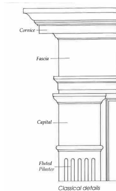
Fig. 6 Classical shop front details
